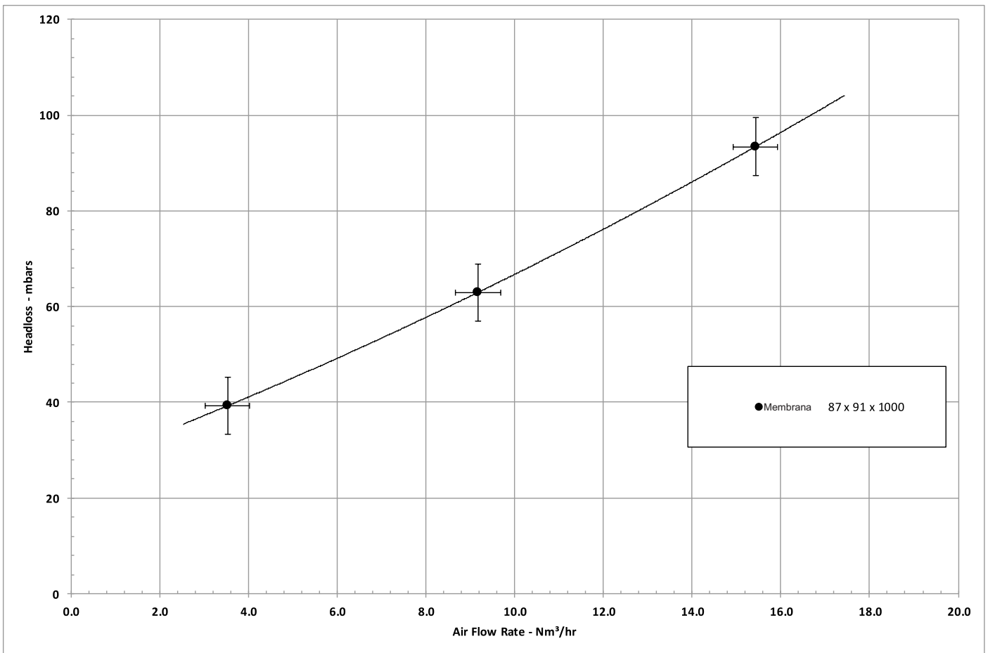
Figure 9 Nm 3 /h v Headloss
