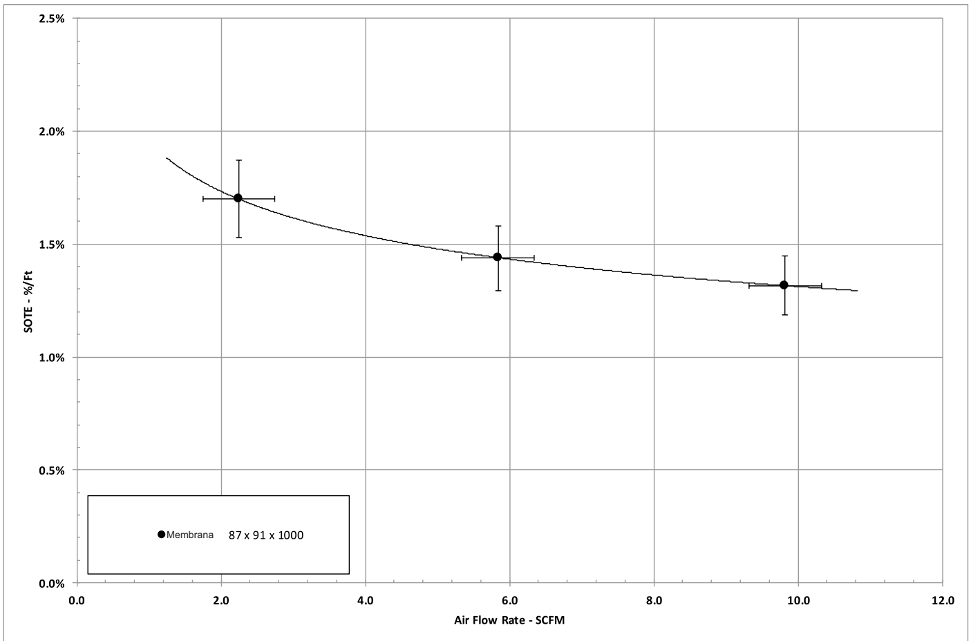
Figure 4 SCFM v SOTE
