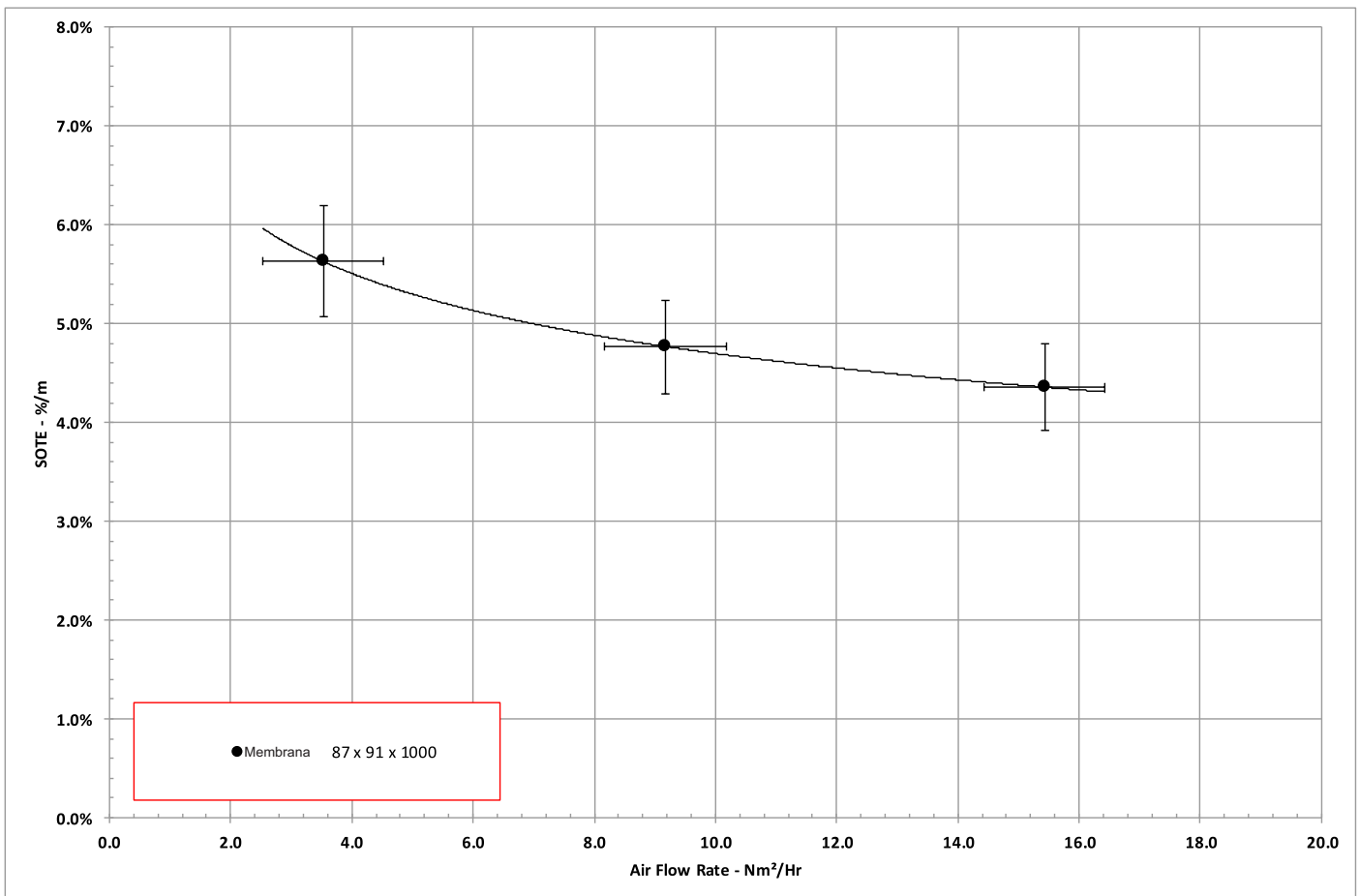
Figure 5 Nm³/h v SOTE
